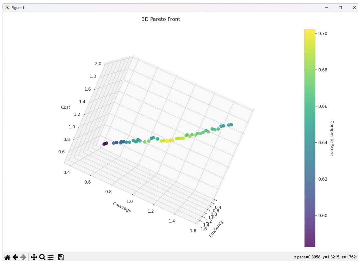
Figure 1. Pareto front in 3D format, formed as a result of applying the hybrid method
