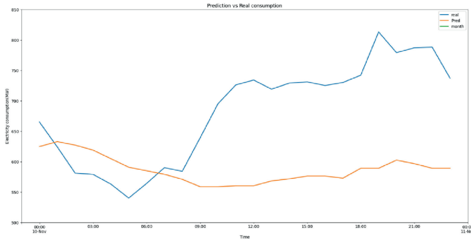
Figure 10. Prediction vs real consumption (10-Nov. 2020y.) by Neural Network Model (86.06%)
